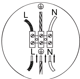
2. Expanded wiring diagram
