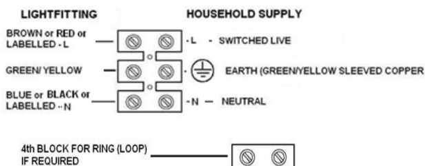
Details of terminal wiring.
