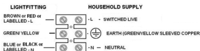
Wiring Details
