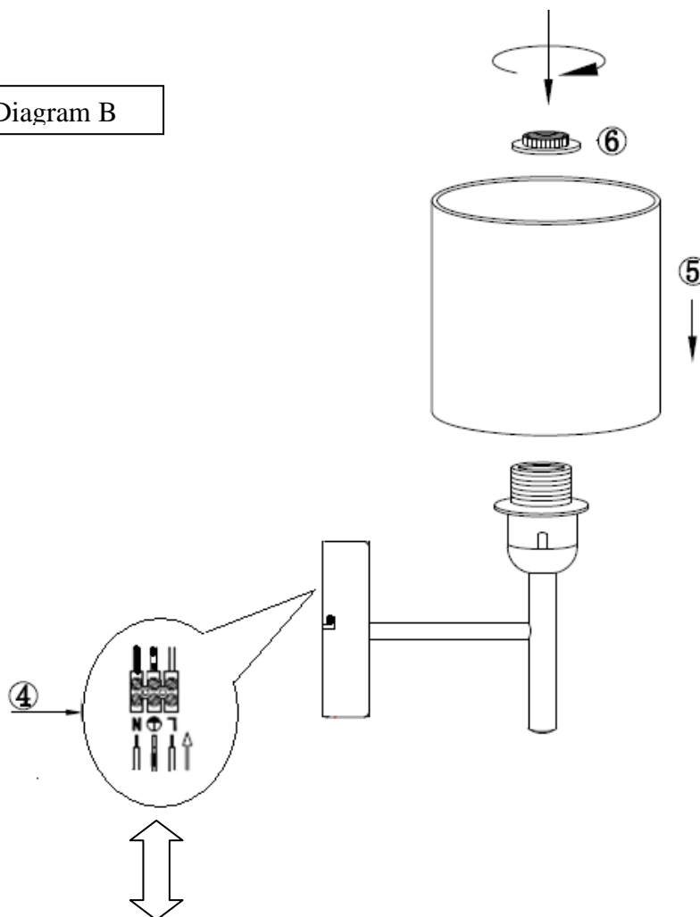
Wiring Details
