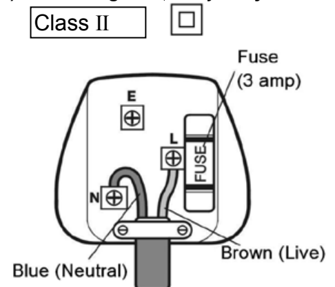
Plug Wiring Diagram
