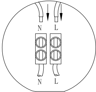
2. Expanded wiring diagram
